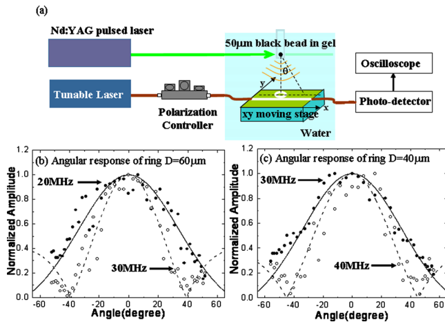
FIG. 3. (Color online) (a) Experimental setup to measure the angular response of the polymer microring, experimental data (dot) and theoretical calculation (line) of angular response of the polymer microrings with D=60\ \mu\text{m} at 20 MHz (solid dot and line) and 30 MHz (empty dot and dashed line) (b), and with D=40\ \mu\text{m} at 30 MHz (solid dot and line) and 40 MHz (empty dot and dashed line) (c).
