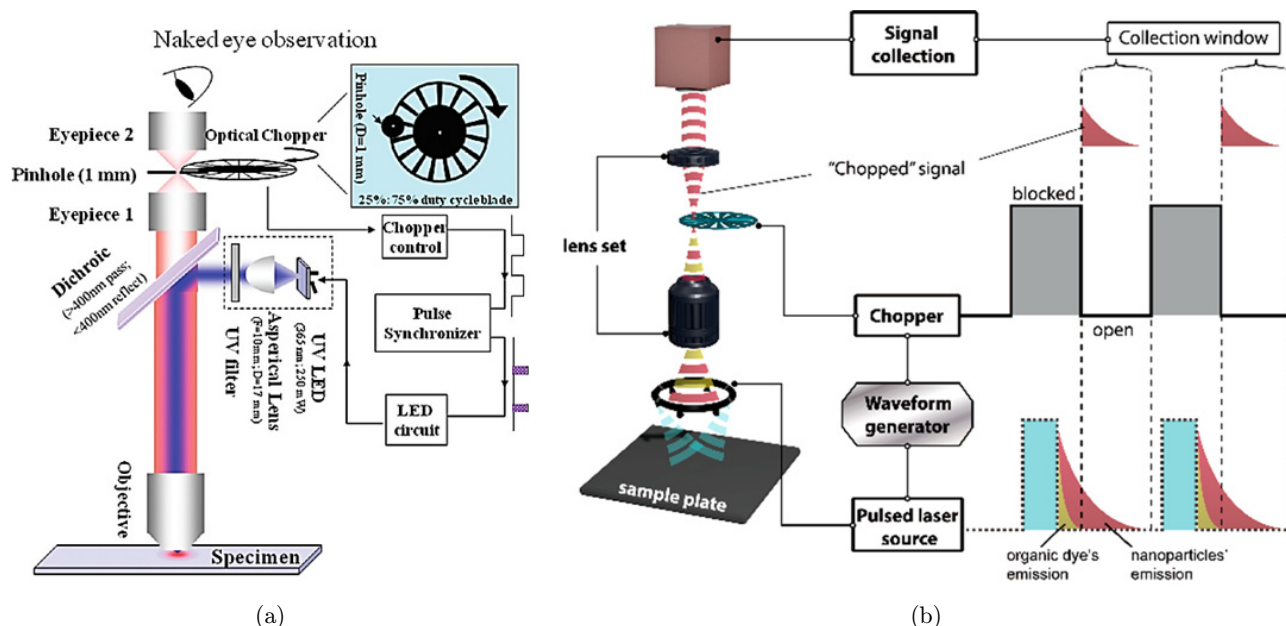
Fig. 5. Example of OC-(iii). (a) Synchronization output was provided by the clock signal from the chopper controller, producing TTL signals to trigger the UV LED circuit, so that an appropriate TG delay can be achieved. (b) Synchronization output was provided by the waveform generator, producing TTL signals that were synchronized with the chopper and were used to synchronize the laser source. An appropriate TG delay can be achieved by setting parameters such as the duty cycle and the initial phase of the TTL signals. Reprinted with permission from Refs. 32 and 48.
